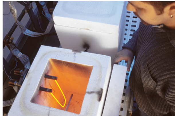
Life test of 4 mm wire.
